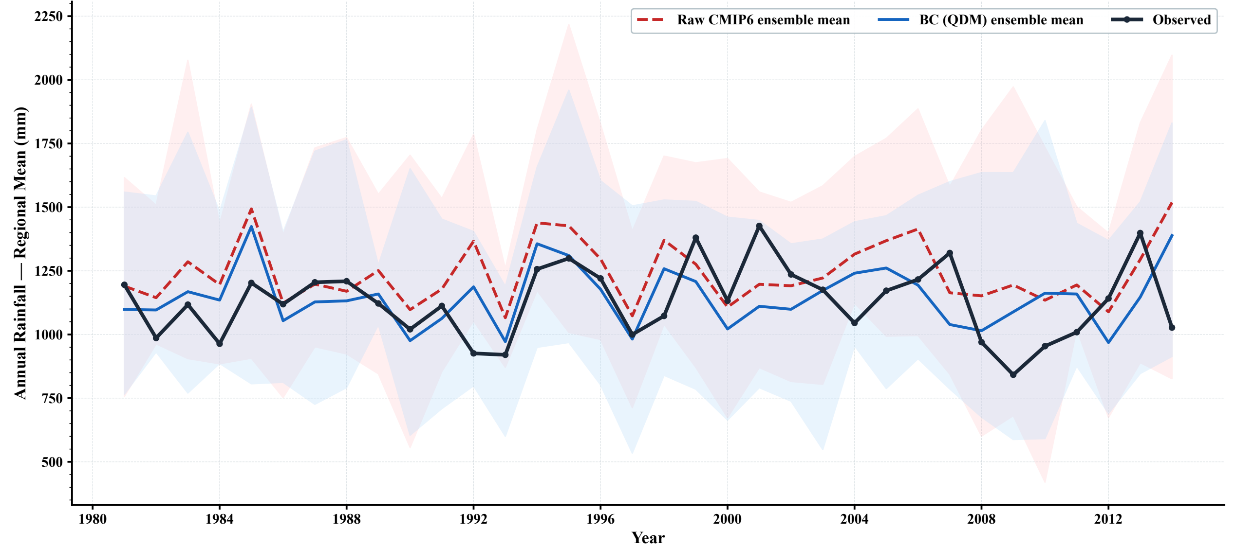
Figure 10 Annual Rainfall Time Series — Regional Mean | 1981–2014 Shaded band = model ensemble range (min–max)
